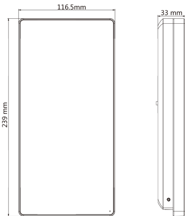
Figure D-2 Device without Fingerprint Module
