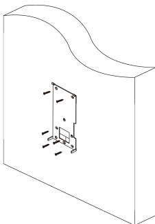
Figure 3-9 Install Mounting Plate
