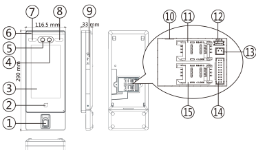
Figure 2-1 Face Recognition Terminal Diagram
