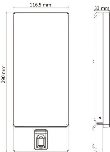
Figure D-1 Device with Fingerprint Module
