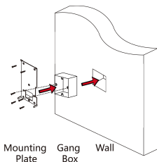
Figure 3-2 Install Mounting Plate
