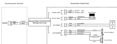
Figure 4-3 Secure Door Control Unit Wiring
