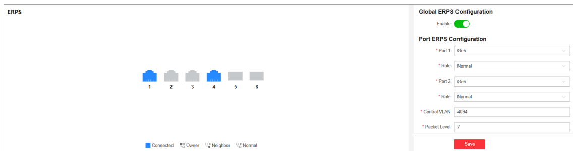
Figure 4-12 Configure ERPS
