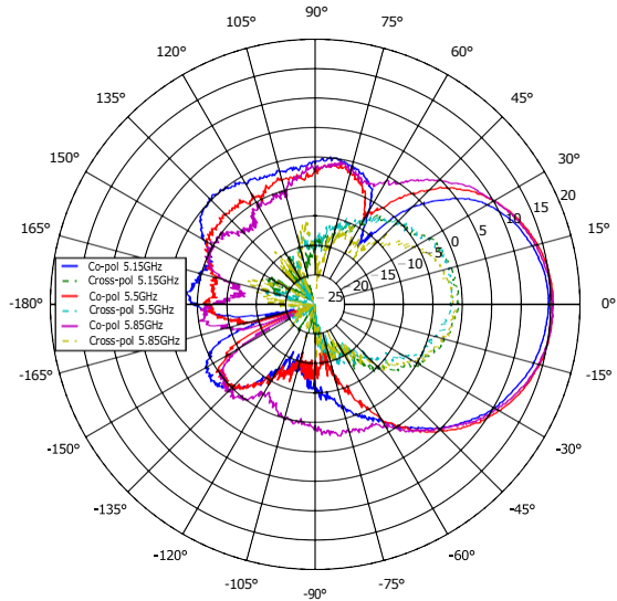
Azimuth, Horizontal
