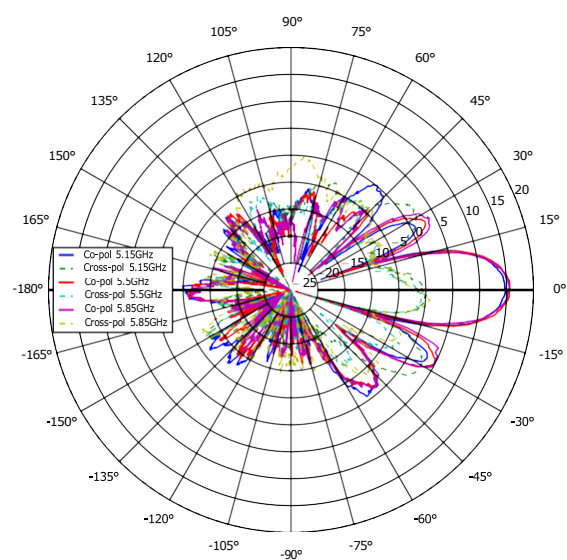
Elevation, Vertical
