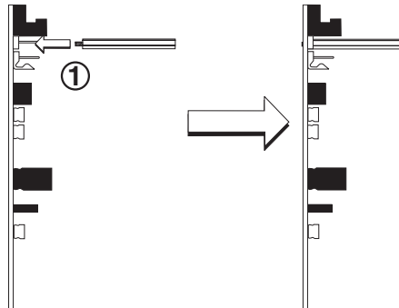
Figure 6a. Installation of XP10-M module in a rear chassis position, method two:
