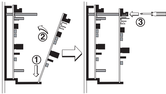
Figure 6b. Installation of XP10-M module in front chassis position:
