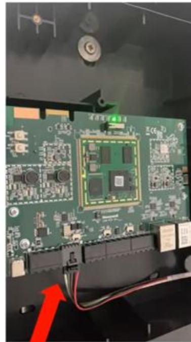
Puerto NUP Tarjeta CLSS Gateway
