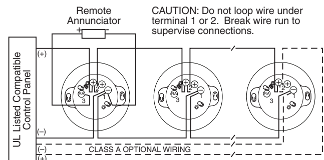
FIGURE 2. WIRING DIAGRAM
