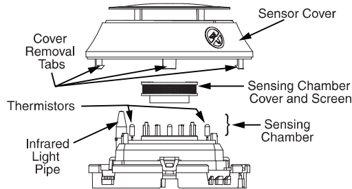
FIGURE 4. CLEANING THE FIRE/CO DETECTOR
