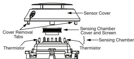
FIGURE 4. CLEANING THE PHOTO/HEAT DETECTOR
