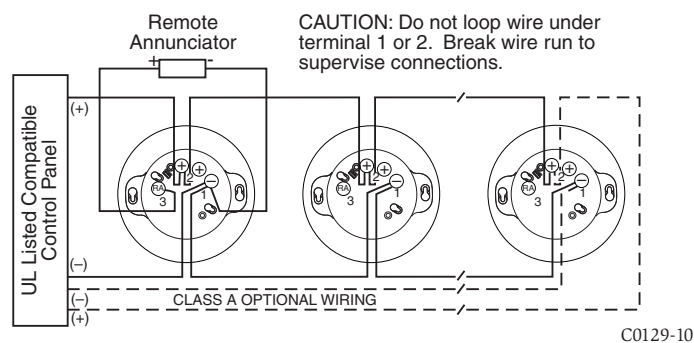
FIGURE 2. WIRING DIAGRAM
