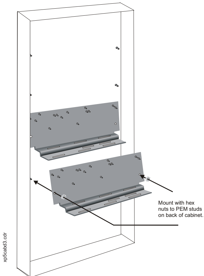
Installation in a CAB-3/CAB-4 Series Cabinet (a CAB-D3/CAB-D4 is shown here)
