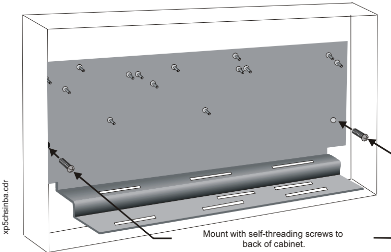
Installation in a BB-25 Cabinet
