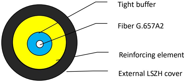
Figure. Cable section (Tip-A)
